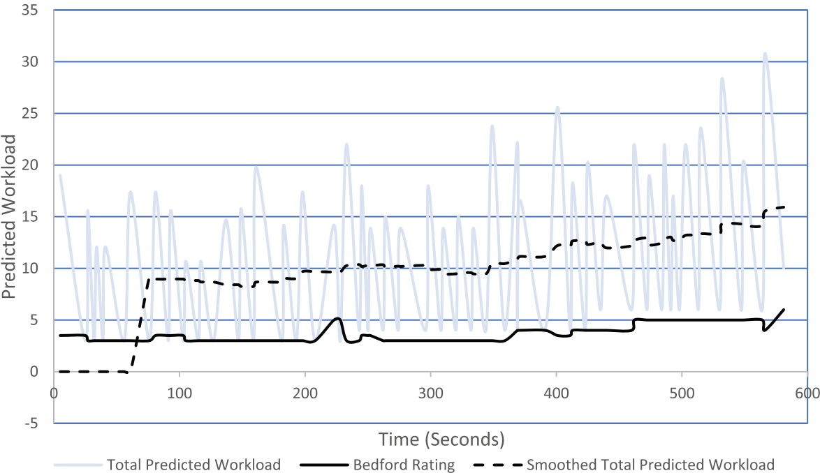
Figure 2. Manual approach segment (under auto-thrust) predictive workload model output (presented both as individual task predicted workload ratings and smoothed workload ratings) plotted against corresponding Bedford scale workload rating data.
