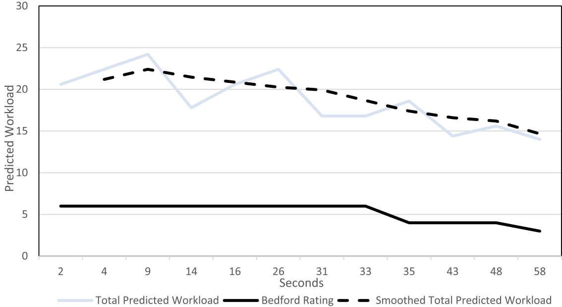
Figure 3. Roll-out flight segment predictive workload model output (presented both as individual task predicted workload ratings and smoothed workload ratings) plotted against corresponding Bedford workload rating data.
